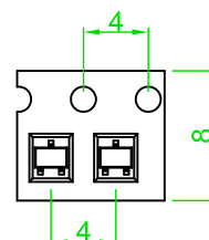
Refer to EIAJ NO. SC-70
