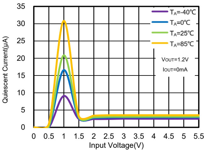
Figure 33. WR0338-12A50R Quiescent Current vs. V IN & Ambient Temperature
