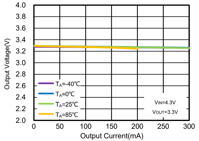
Figure 56. WR0338-33A20R Output Voltage vs. I OUT & Ambient Temperature
