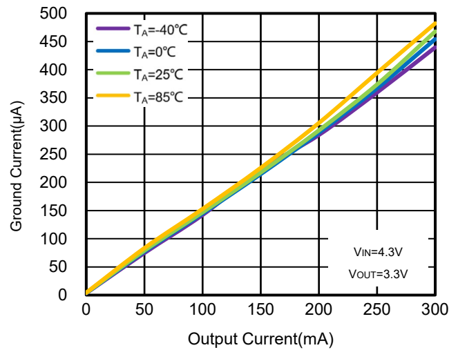
Figure 44. WR0338-33A20R Ground Pin Current vs. I OUT & Ambient Temperature
