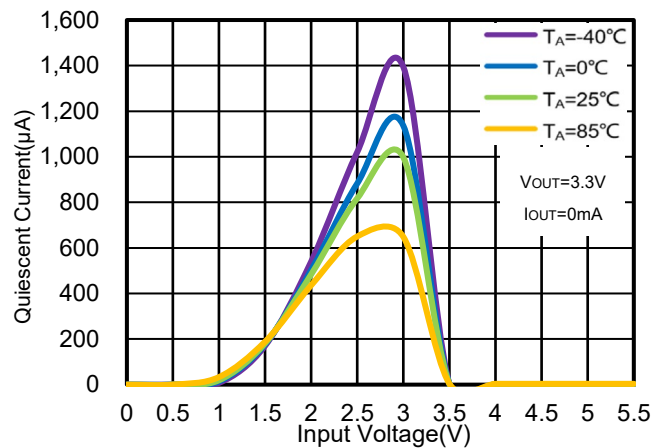
Figure 27. WR0338-33A20R Quiescent Current vs. V IN & Ambient Temperature
