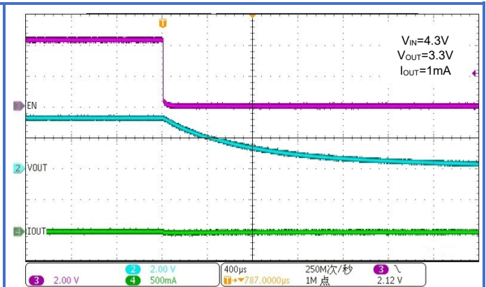
Figure 62. WR0338-33A50R EN Shutdown
