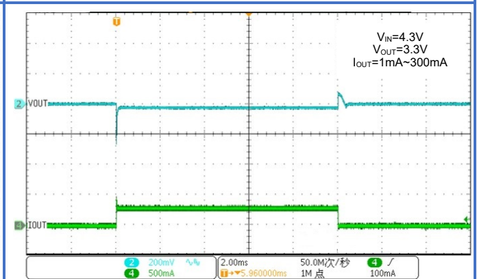
Figure 66. WR0338-33A50R Load Transient
