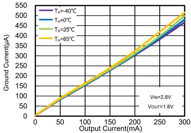
Figure 45. WR0338-18A50R Ground Pin Current vs. I OUT & Ambient Temperature
