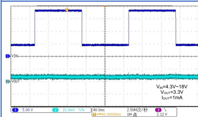
Figure 65. WR0338-33A50R Line Transient
