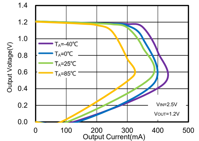
Figure 42. WR0338-12A20R Foldback Current Limit vs. I OUT & Ambient Temperature
