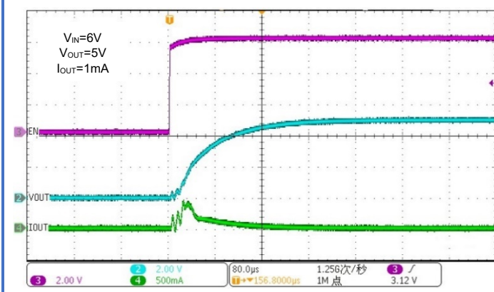
Figure 63. WR0338-50A50R Soft Start from EN
