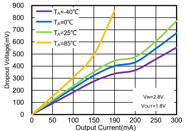
Figure 52. WR0338-18A20R Dropout Voltage vs. I OUT & Ambient Temperature
