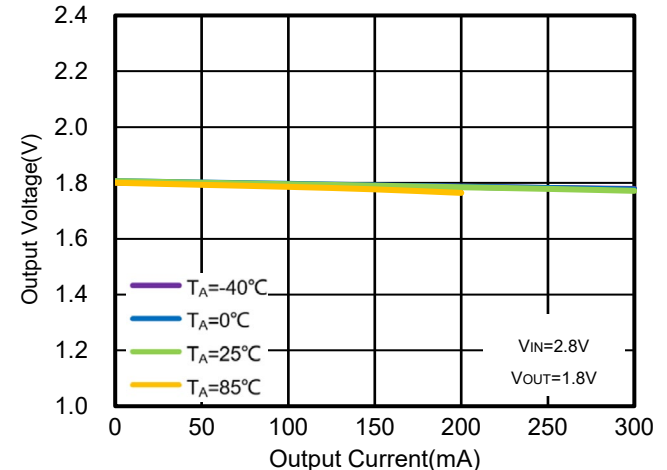
Figure 58. WR0338-18A20R Output Voltage vs. I OUT & Ambient Temperature
