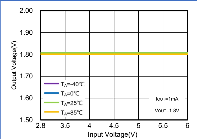
Figure 16. WR0338-18A20R Regulation vs. V IN (Line Regulation) & Ambient Temperature
