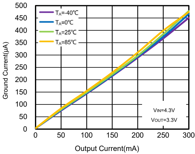
Figure 43. WR0338-33A50R Ground Pin Current vs. I OUT & Ambient Temperature
