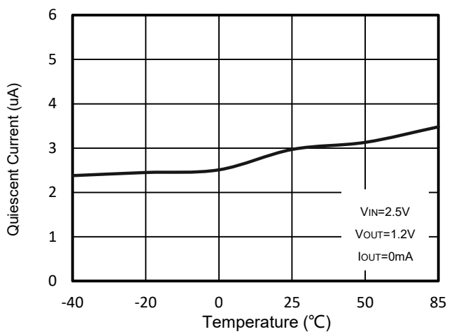
Figure 12. WR0338-12A20R Quiescent Current vs. Ambient Temperature
