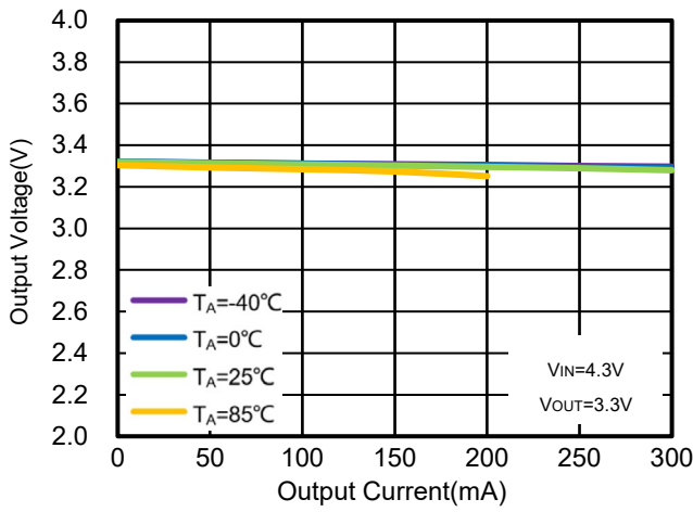
Figure 55. WR0338-33A50R Output Voltage vs. I OUT & Ambient Temperature
