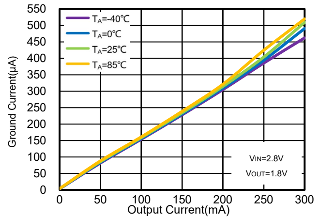
Figure 46. WR0338-18A20R Ground Pin Current vs. I OUT & Ambient Temperature
