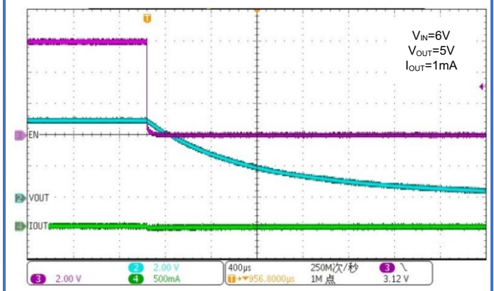
Figure 64. WR0338-50A50R EN Shutdown
