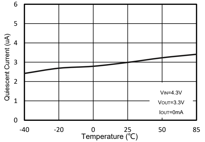
Figure 2. WR0338-33A50R Quiescent Current vs. Ambient Temperature
