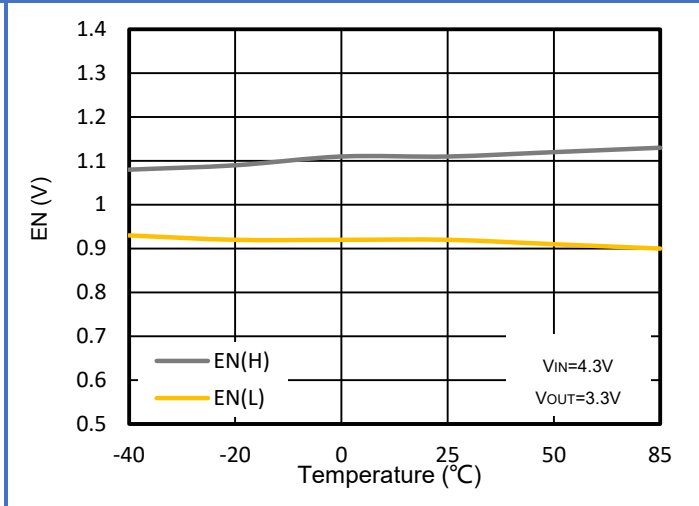
Figure 22. WR0338-33A50R Enable Threshold vs. Ambient Temperature
