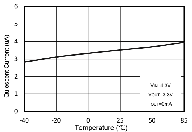
Figure 4. WR0338-33A20R Quiescent Current vs. Ambient Temperature
