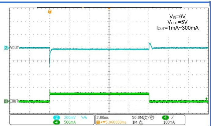
Figure 68. WR0338-50A50R Load Transient
