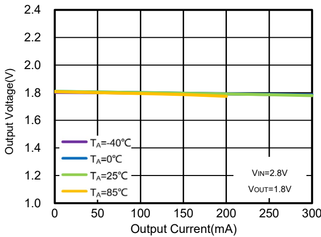
Figure 57. WR0338-18A50R Output Voltage vs. I OUT & Ambient Temperature
