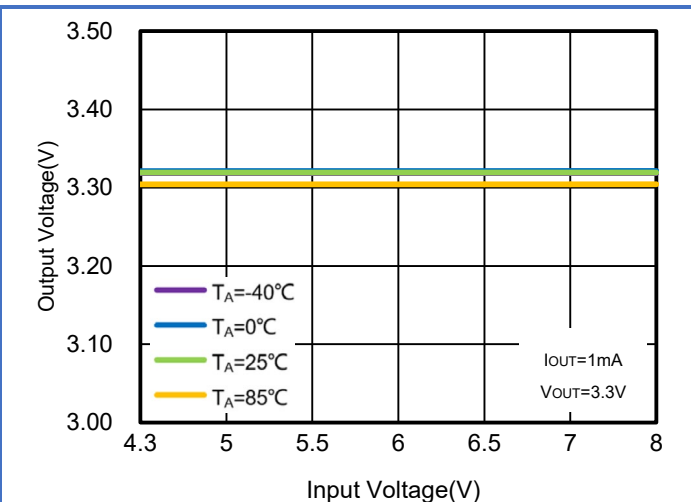
Figure 14. WR0338-33A20R Regulation vs. V IN (Line Regulation) & Ambient Temperature
