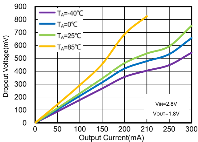
Figure 51. WR0338-18A50R Dropout Voltage vs. I OUT & Ambient Temperature
