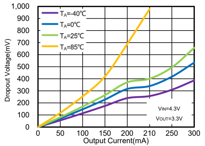
Figure 50. WR0338-33A20R Dropout Voltage vs. I OUT & Ambient Temperature
