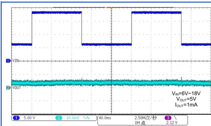
Figure 67. WR0338-50A50R Line Transient
