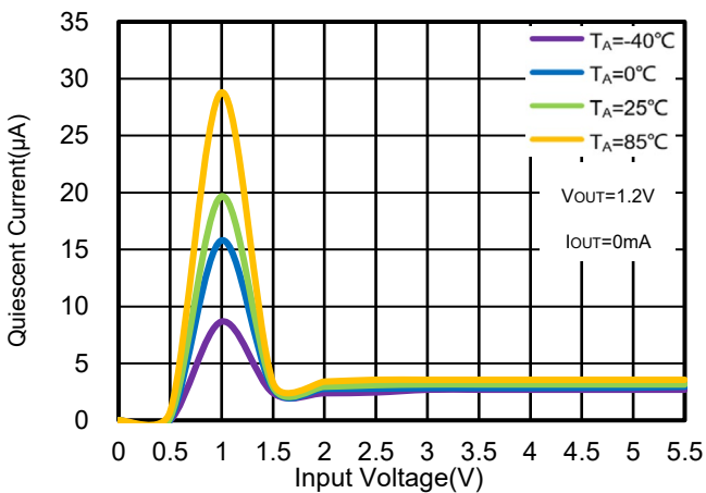
Figure 35. WR0338-12A20R Quiescent Current vs. V IN & Ambient Temperature
