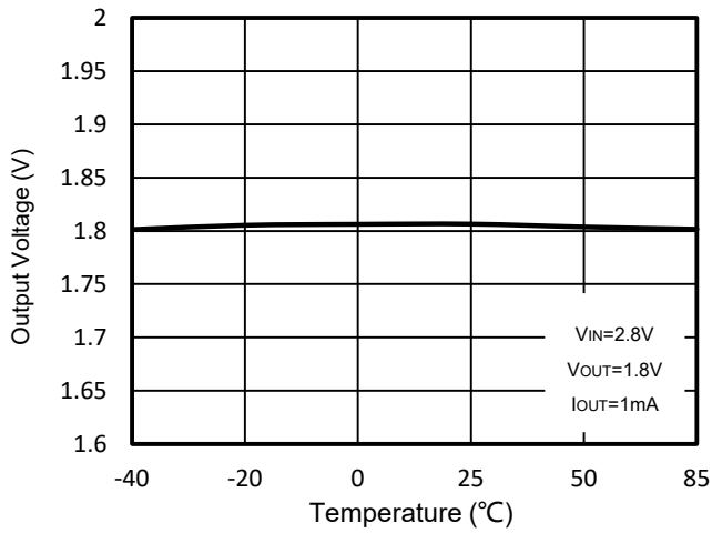
Figure 7. WR0338-18A20R Output Voltage vs. Ambient Temperature
