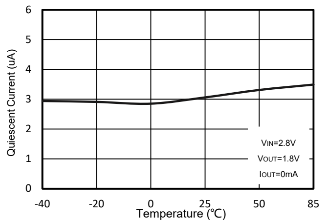
Figure 6. WR0338-18A50R Quiescent Current vs. Ambient Temperature
