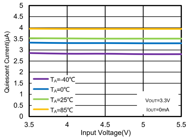
Figure 26. WR0338-33A50R Quiescent Current vs. V IN & Ambient Temperature
