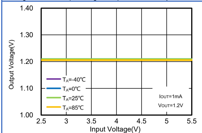
Figure 17. WR0338-12A50R Regulation vs. V IN (Line Regulation) & Ambient Temperature
