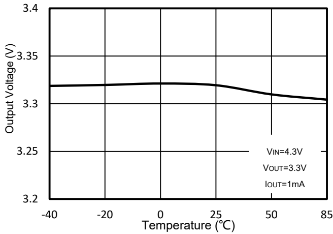
Figure 1. WR0338-33A50R Output Voltage vs. Ambient Temperature
