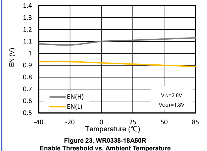
Figure 23. WR0338-18A50R Enable Threshold vs. Ambient Temperature
