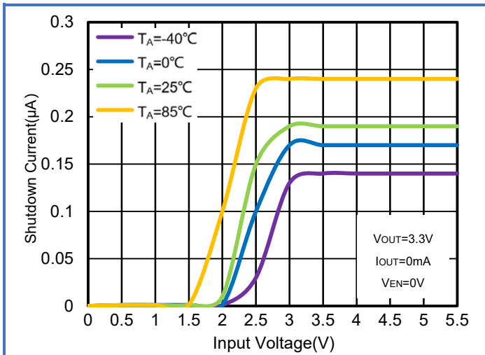
Figure 19. WR0338-33A50R Shutdown Current vs. V IN & Ambient Temperature
