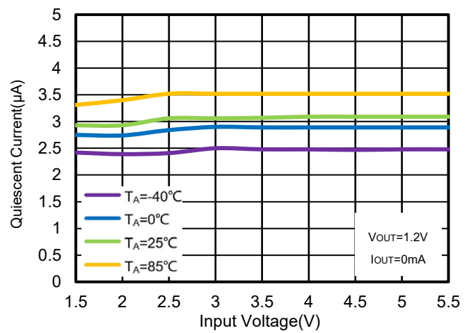
Figure 34. WR0338-12A50R Quiescent Current vs. V IN & Ambient Temperature
