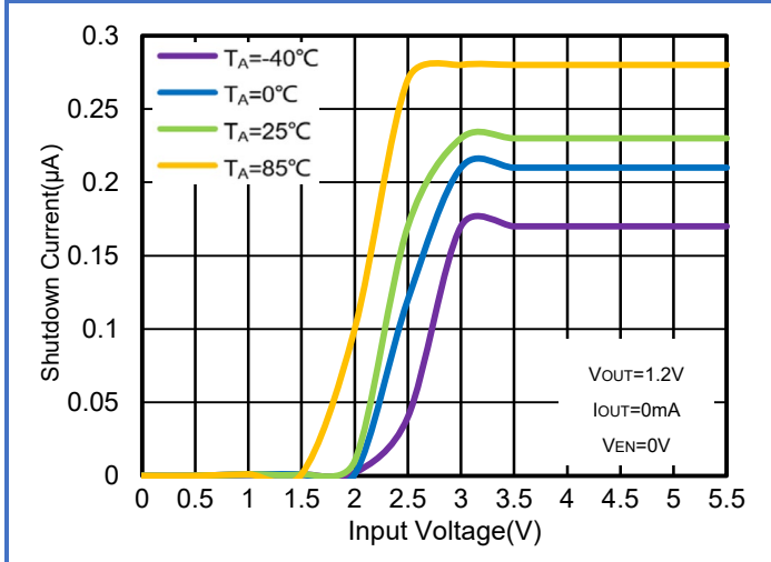
Figure 21. WR0338-12A50R Shutdown Current vs. V IN & Ambient Temperature
