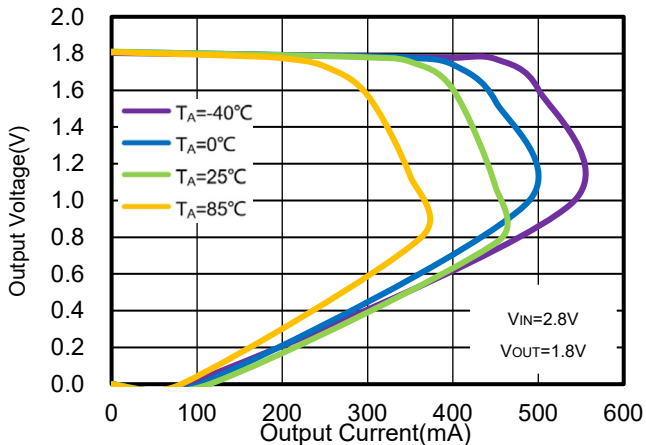
Figure 39. WR0338-18A50R Foldback Current Limit vs. I OUT & Ambient Temperature
