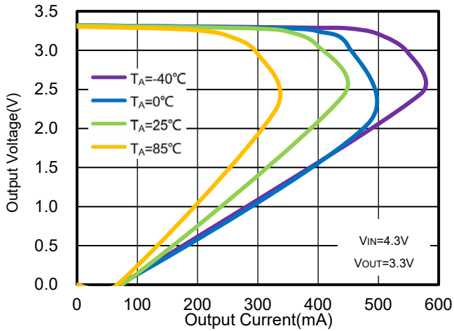
Figure 37. WR0338-33A50R Foldback Current Limit vs. I OUT & Ambient Temperature
