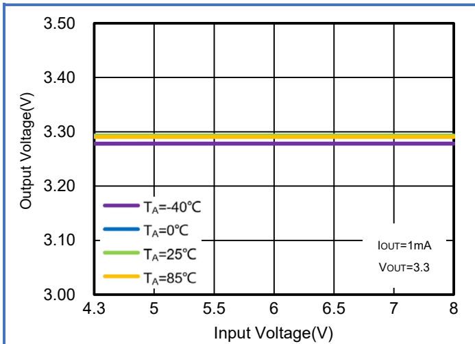
Figure 13. WR0338-33A50R Regulation vs. V IN (Line Regulation) & Ambient Temperature
