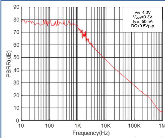
Figure 69. WR0338-33A50R Power Supply Rejection Ratio vs. Frequency
