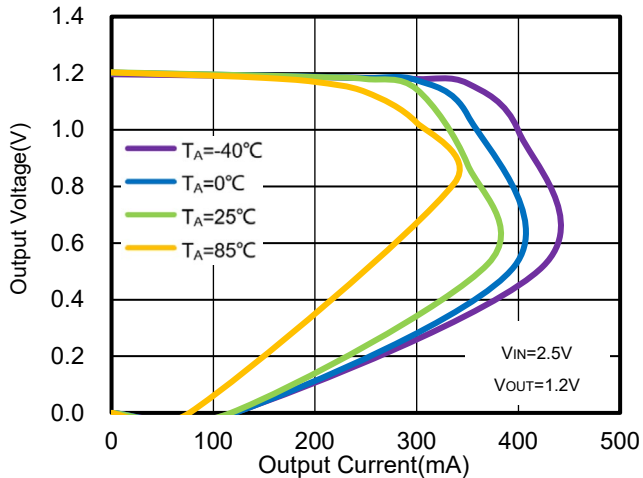
Figure 41. WR0338-12A50R Foldback Current Limit vs. I OUT & Ambient Temperature
