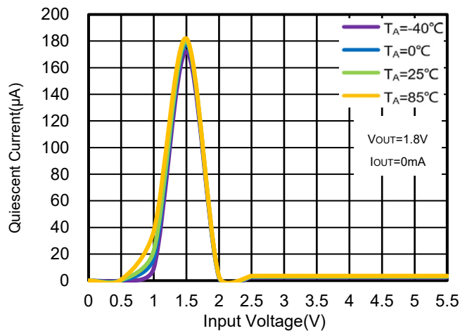
Figure 29. WR0338-18A50R Quiescent Current vs. V IN & Ambient Temperature
