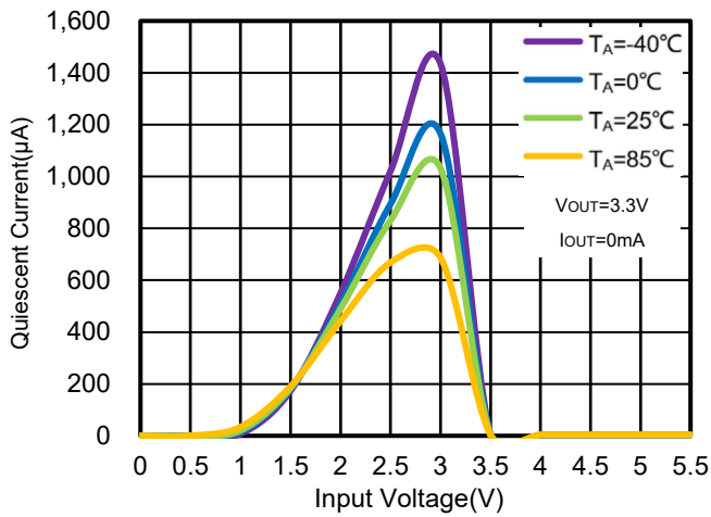
Figure 25. WR0338-33A50R Quiescent Current vs. V IN & Ambient Temperature
