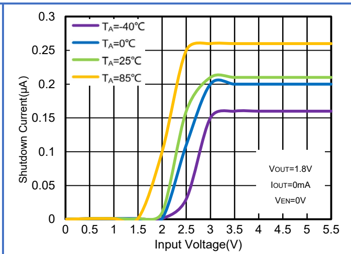
Figure 20. WR0338-18A50R Shutdown Current vs. V IN & Ambient Temperature
