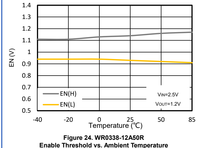
Figure 24. WR0338-12A50R Enable Threshold vs. Ambient Temperature
