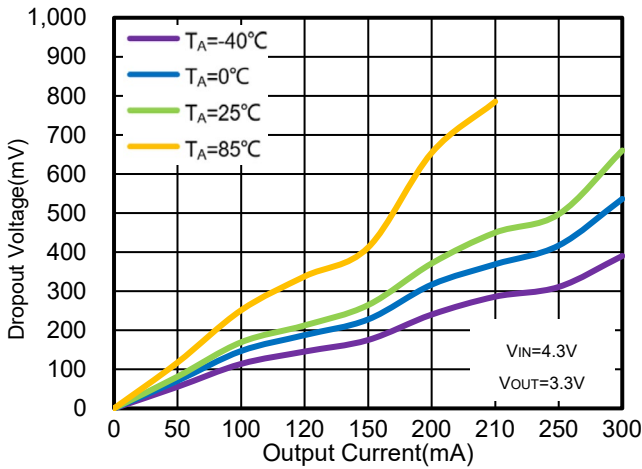
Figure 49. WR0338-33A50R Dropout Voltage vs. I OUT & Ambient Temperature
