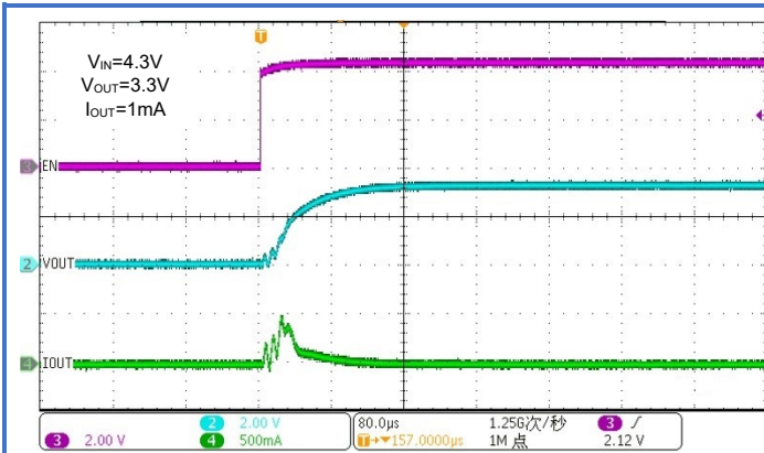
Figure 61. WR0338-33A50R Soft Start from EN
