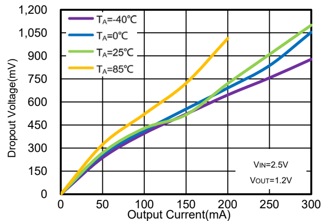
Figure 54. WR0338-12A20R Dropout Voltage vs. I OUT & Ambient Temperature
