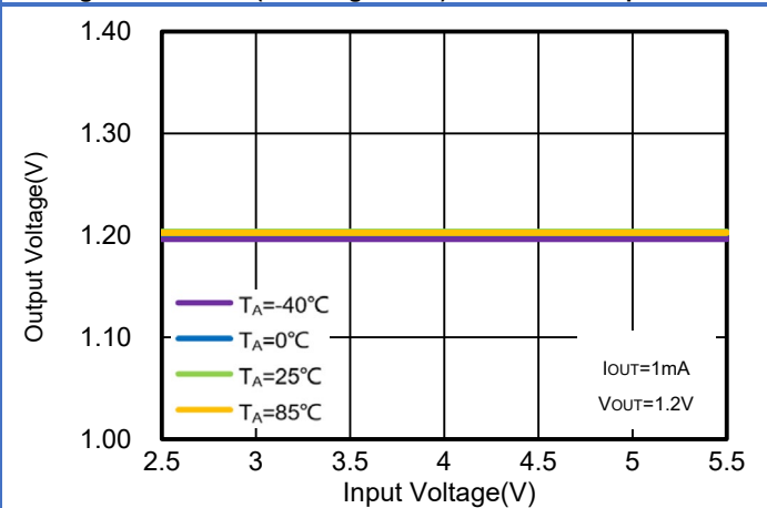
Figure 18. WR0338-12A20R Regulation vs. V IN (Line Regulation) & Ambient Temperature
