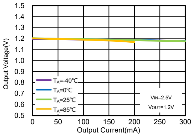
Figure 59. WR0338-12A50R Output Voltage vs. I OUT & Ambient Temperature
