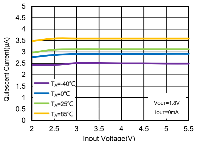
Figure 30. WR0338-18A50R Quiescent Current vs. V IN & Ambient Temperature
