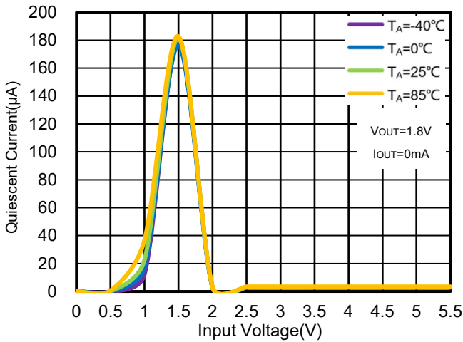
Figure 31. WR0338-18A20R Quiescent Current vs. V IN & Ambient Temperature
