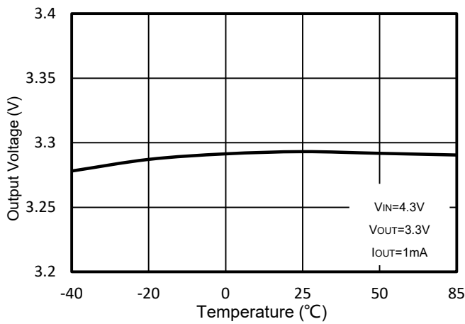
Figure 3. WR0338-33A20R Output Voltage vs. Ambient Temperature
