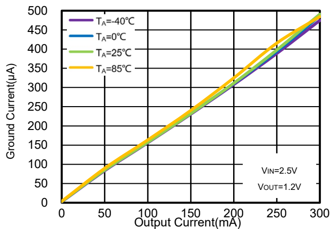
Figure 48. WR0338-12A20R Ground Pin Current vs. I OUT & Ambient Temperature
