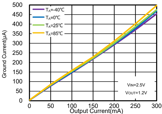
Figure 47. WR0338-12A50R Ground Pin Current vs. I OUT & Ambient Temperature
