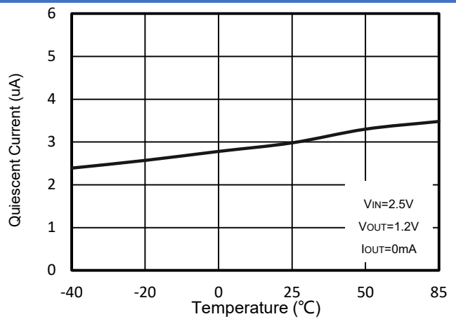
Figure 10. WR0338-12A50R Quiescent Current vs. Ambient Temperature
