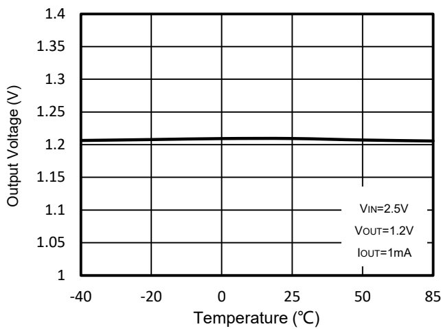
Figure 11. WR0338-12A20R Output Voltage vs. Ambient Temperature
