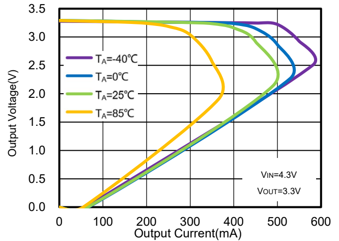
Figure 38. WR0338-33A20R Foldback Current Limit vs. I OUT & Ambient Temperature
