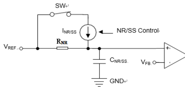
Soft-Start Circuit
