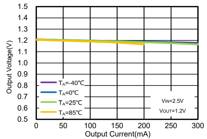
Figure 60. WR0338-12A20R Output Voltage vs. I OUT & Ambient Temperature
