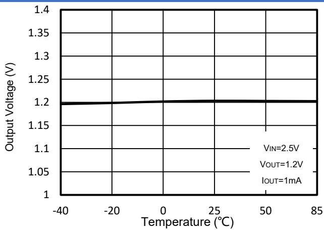
Figure 9. WR0338-12A50R Output Voltage vs. Ambient Temperature
