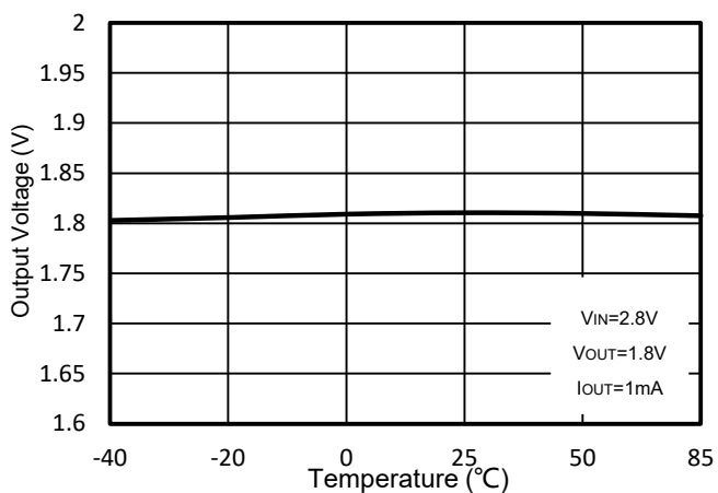
Figure 5. WR0338-18A50R Output Voltage vs. Ambient Temperature
