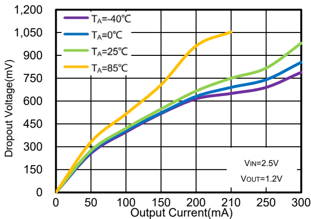
Figure 53. WR0338-12A50R Dropout Voltage vs. I OUT & Ambient Temperature
