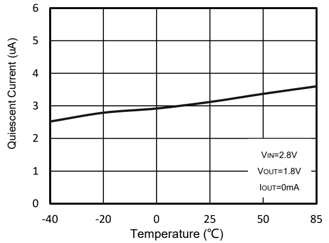
Figure 8. WR0338-18A20R Quiescent Current vs. Ambient Temperature
