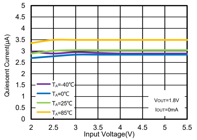
Figure 32. WR0338-18A20R Quiescent Current vs. V IN & Ambient Temperature
