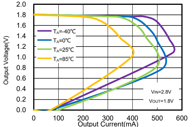
Figure 40. WR0338-18A20R Foldback Current Limit vs. I OUT & Ambient Temperature
