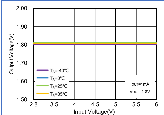
Figure 15. WR0338-18A50R Regulation vs. V IN (Line Regulation) & Ambient Temperature
