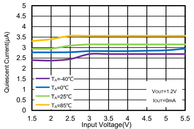
Figure 36. WR0338-12A20R Quiescent Current vs. V IN & Ambient Temperature
