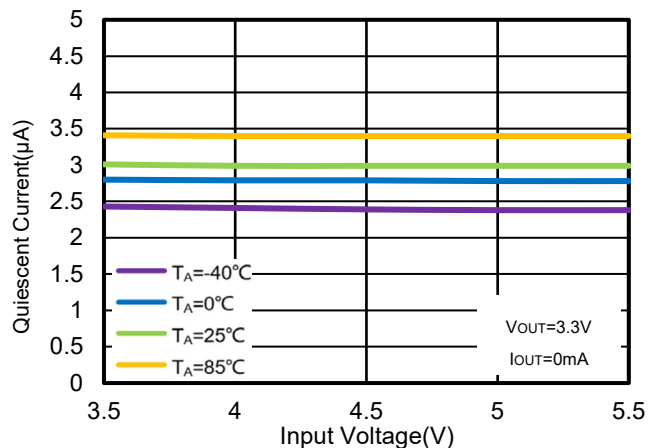
Figure 28. WR0338-33A20R Quiescent Current vs. V IN & Ambient Temperature
