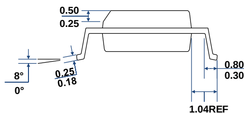
LEFT-SIDE VIEW
